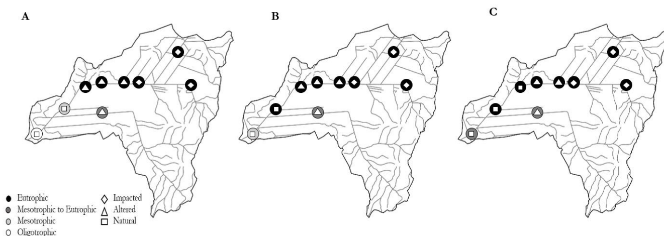
Figure 2. Simplified representation of TRIX (eutrophic, mesotrophic to eutrophic, mesotrophic and oligotrophic) and of RAP (impacted, changed and natural) in the sampling periods, pre-summer (A), summer (B) and post-summer (C). Source: Authors.
