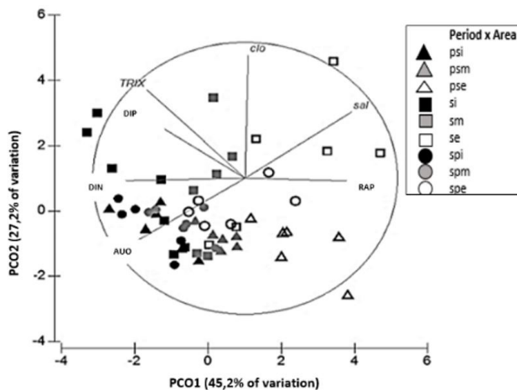
Figure 3. Graphic of the principal coordinates analysis (PCoA) with the variables used in TRIX and RAP equation, by sampling period and area of the Papaquara river. Source: Authors.
